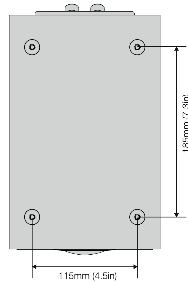
BASE STAND SCREW ALIGNMENT
