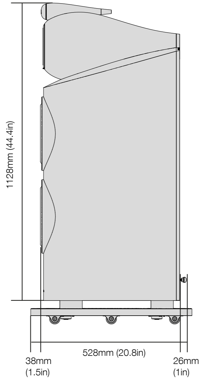
SIDE
