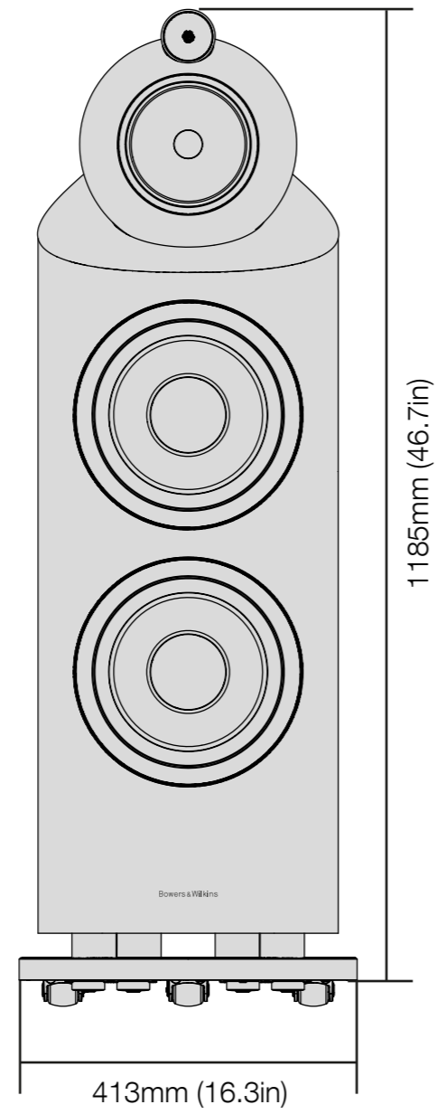
FRONT
