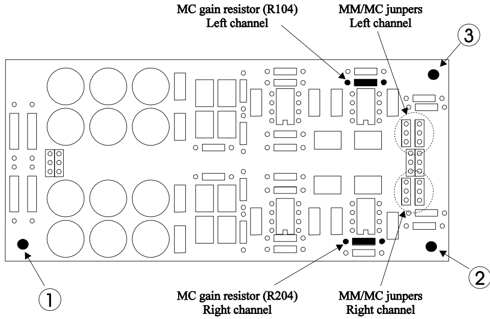
Fig.2 CP-45 Optional Phono Board
