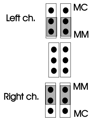
Fig.2a Jumpers setting for MM
