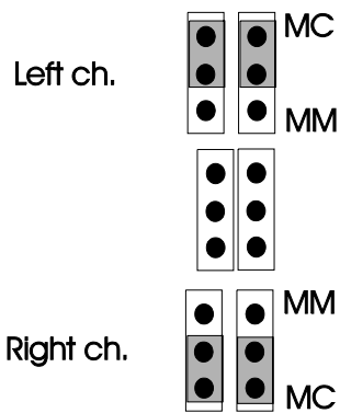
Fig.2a Jumpers setting for MC
