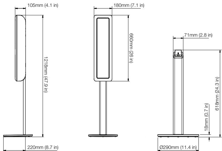
Floor stand
