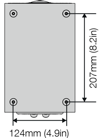
CABINET BASE SCREW ALIGNMENT FOR PLINTH
