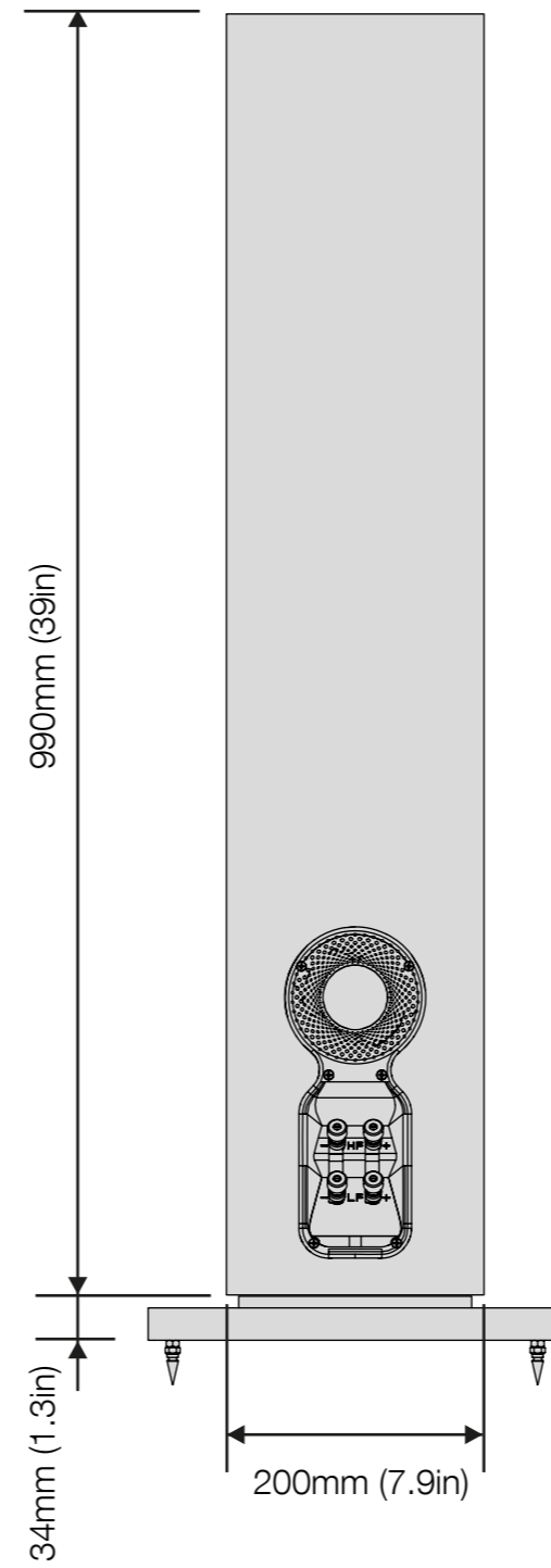
BACK
