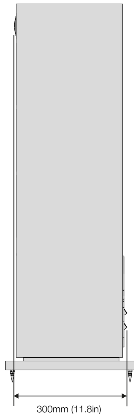
RIGHT SIDE
